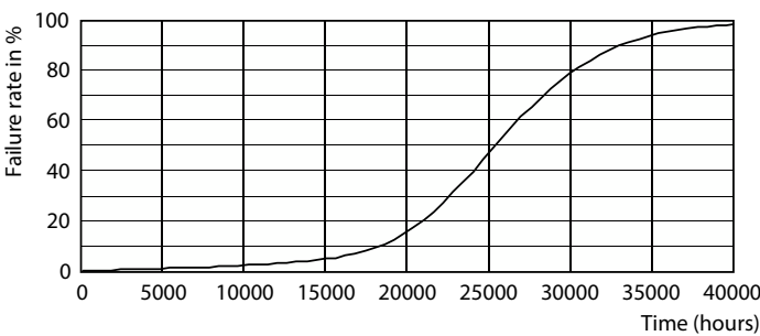
Life Expectancy Diagram - MAS LED spot VLE D 6.2-80W GU10 940 36D
