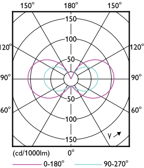
Light Distribution Diagram - CorePro LEDcapsuleLV 1-10W G4 830
