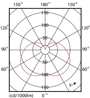
Light Distribution Diagram - CorePro LED Stick ND 9.5-68W T38 E27 830
