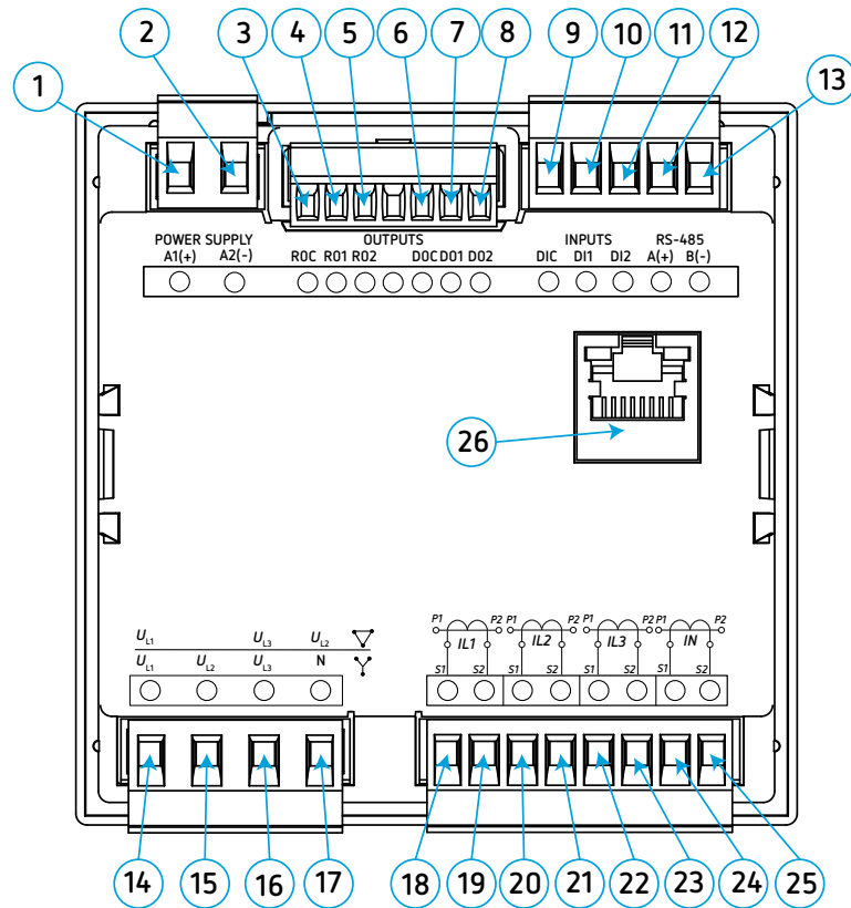
Figura 2: Bornes del CVM-C11-ITF-IN-ETH-ICT2.
