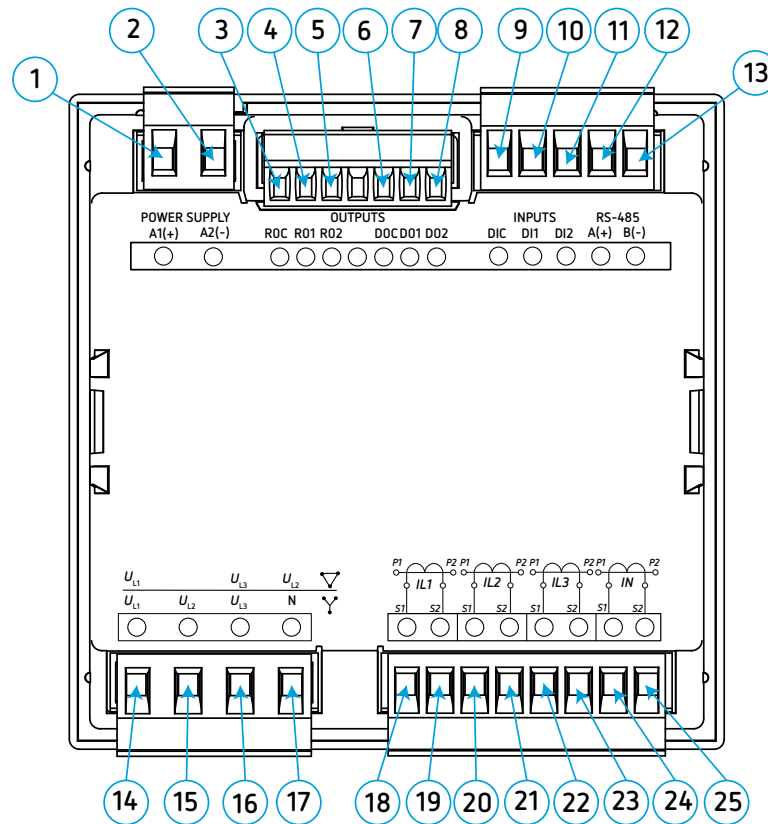
Figura 1: Bornes del CVM-C11-ITF-IN-485-ICT2 y CVM-C11-MC-IN-485-ICT2.
